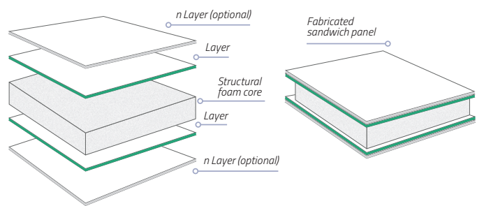
Foam lay-up
