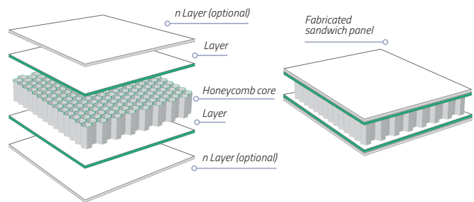
Honeycomb lay-up
